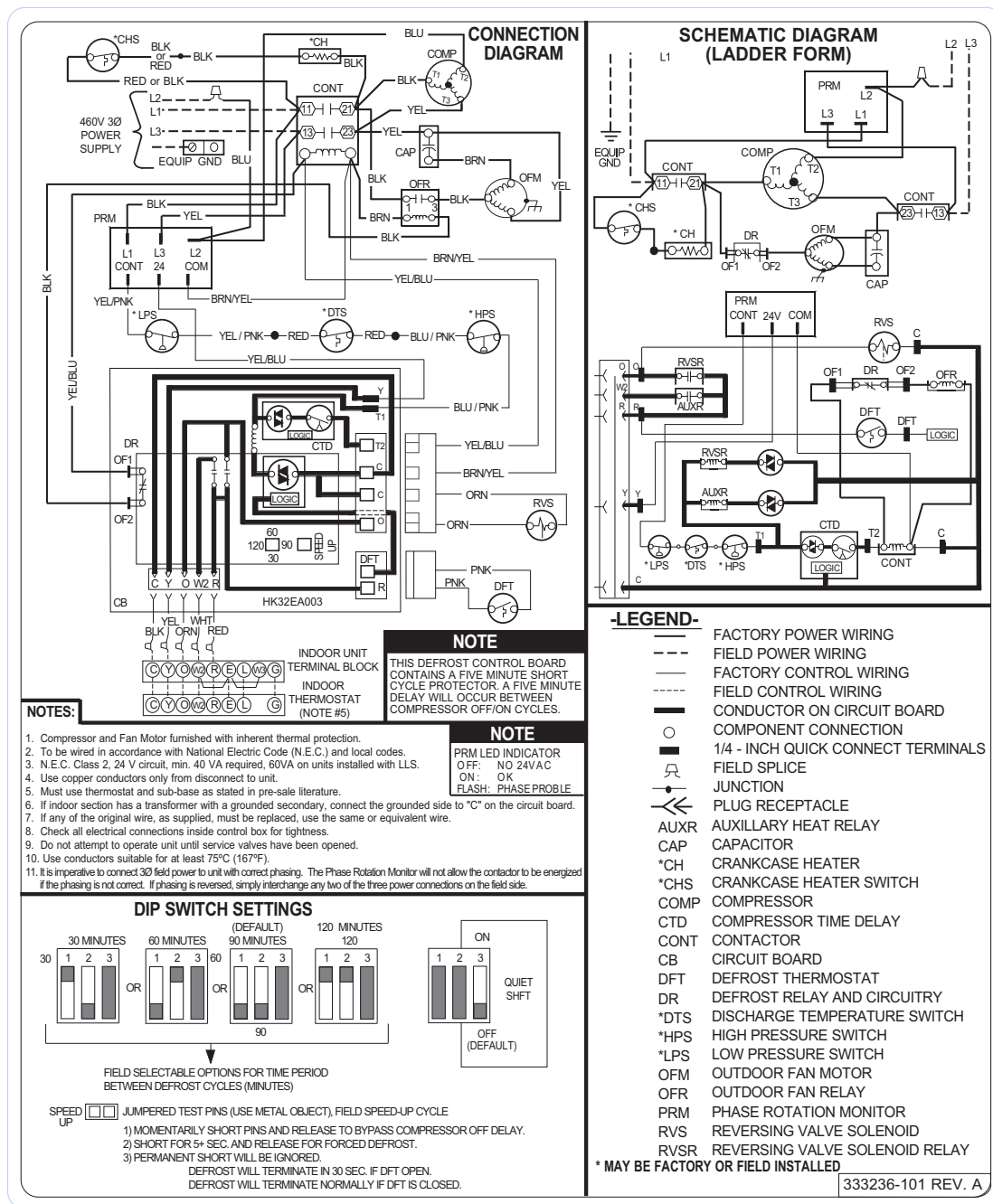
Fig. 3 – Wiring Diagram — Model size 3 - 5 tons, 460/3
