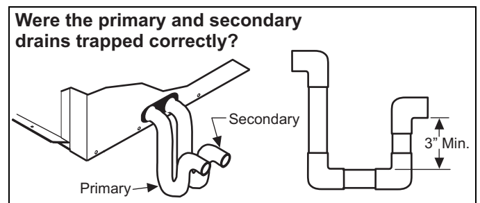
FIGURE 16: Drain Traps
