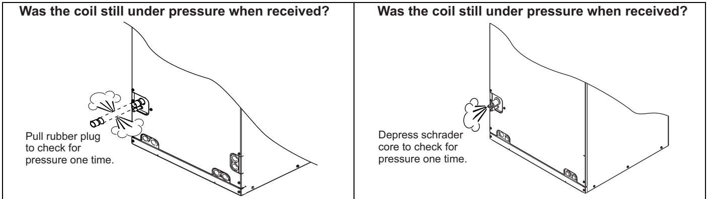
FIGURE 14: Pressure Check
