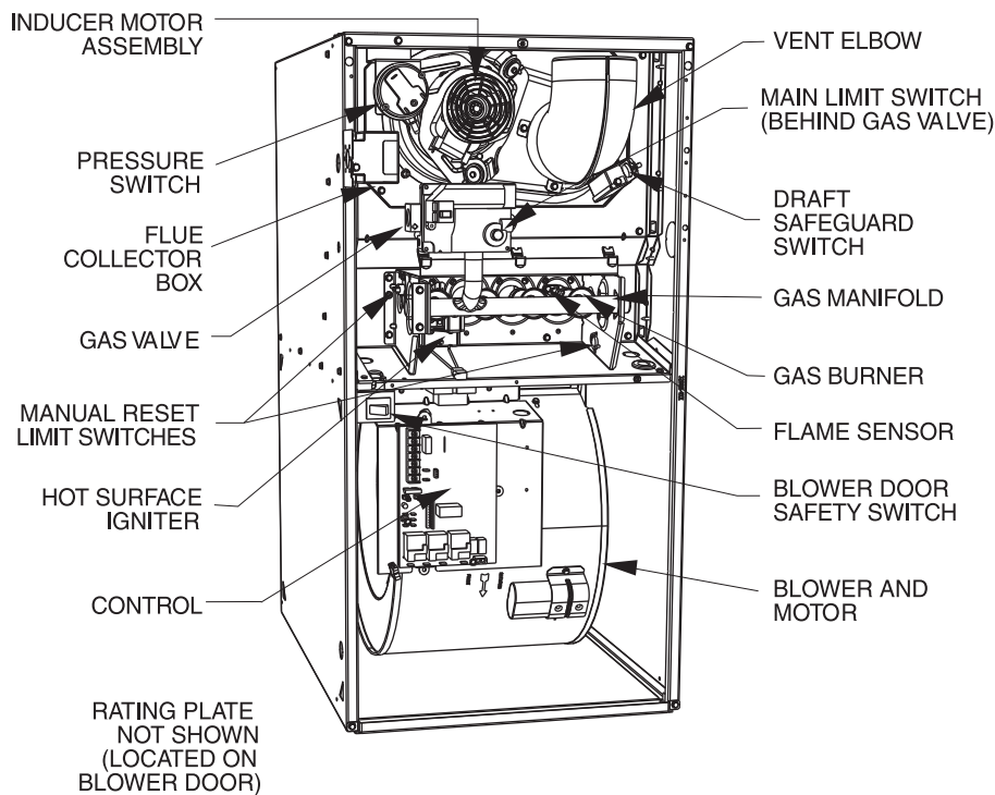
Fig. 17 - Representative Furnace Drawing
