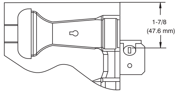
Fig. 26 - Igniter Position - Top View
