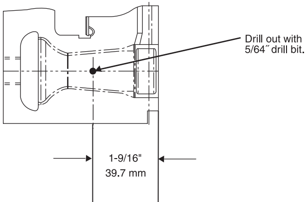
Fig. 24 - Mixer Screw Location
