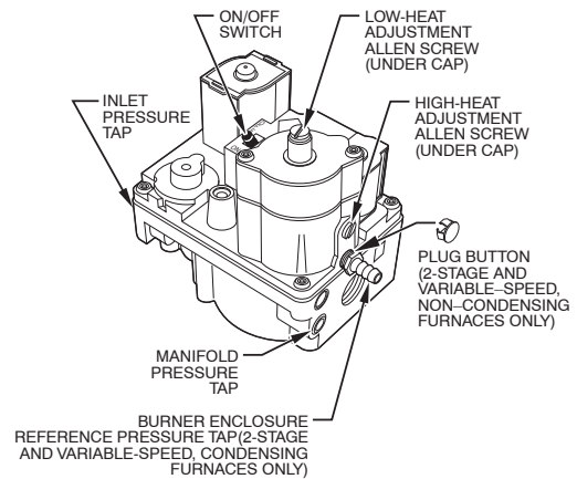
Fig. 29 - 2 Stage E Gas Valve
