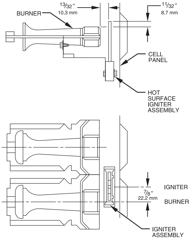
Fig. 27 - Silicon Carbide Igniters
