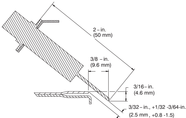
Fig. 9 - Igniter Position - Side View
