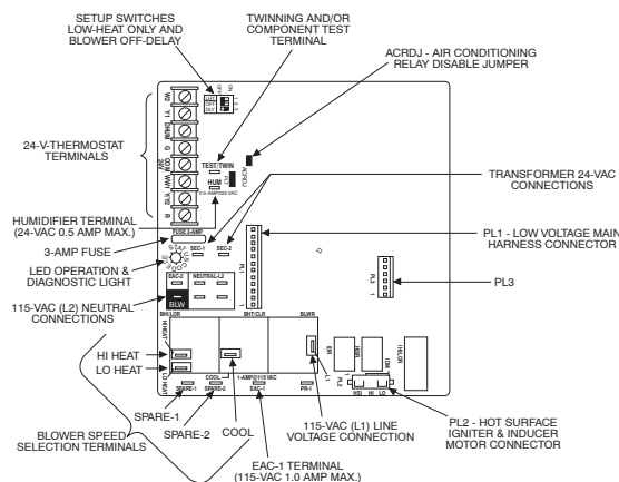
Fig. 32 - 80% Furnace Control Board
