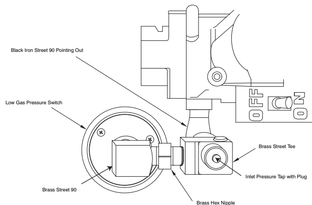
Fig. 11 - Low Gas Pressure Switch - All Widths
