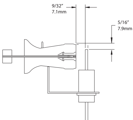
Fig. 25 - Igniter Position - Side View
