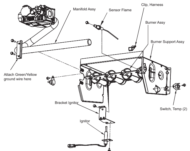
Fig. 18 - 80% Burner
