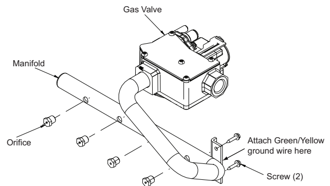
Fig. 19 - 80% Manifold
