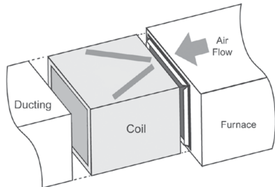
Fig 5B-1. Horizontal Left Application
